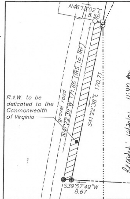
DETAIL OF R.O.W. DEDICATION
